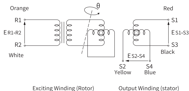
Fig.1 Wiring Diagram
