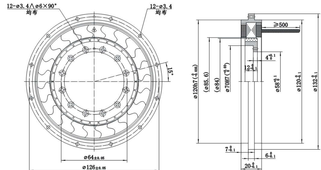
技术图纸 Technical drawings
