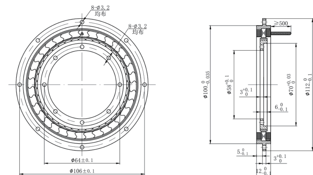
技术图纸 Technical drawings
