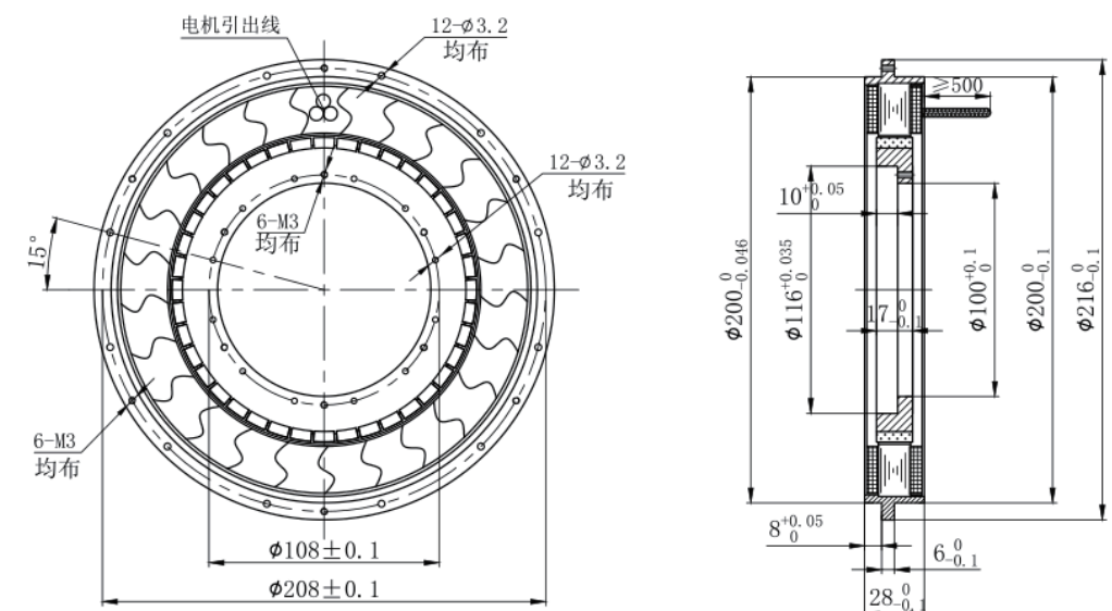
技术图纸 Technical drawings
