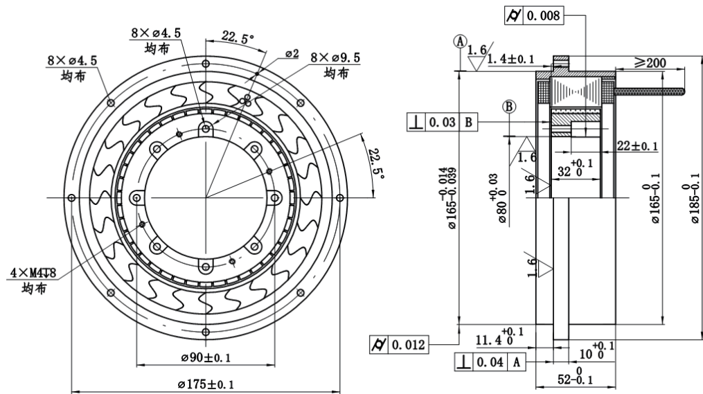
技术图纸 Technical drawings
