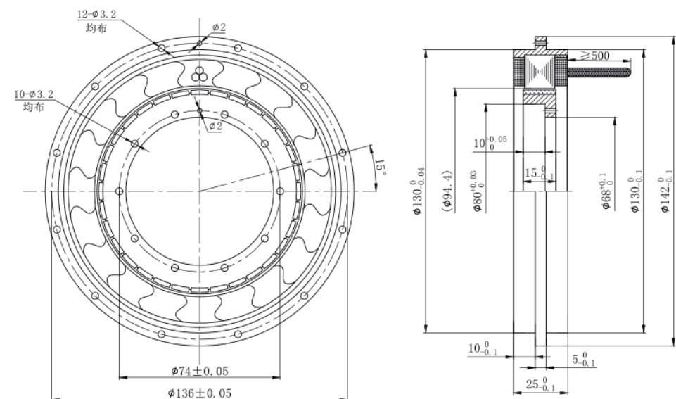
技术图纸 Technical drawings
